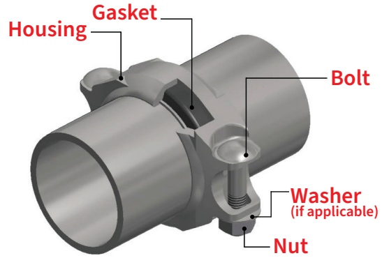
Coupling Assembly
